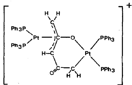
Fig. 13. The dinuclear structure proposed for [\text{Pt}_2(\text{C}_5\text{H}_5\text{O}_2)(\text{PPh}_3)_4]^+ [147].
