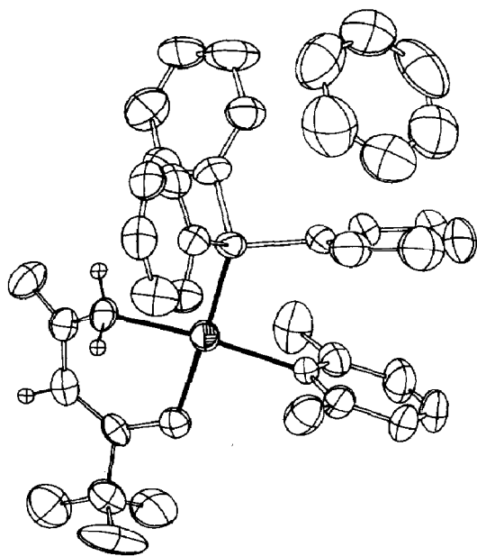
Fig. 11. The molecular structure of [\text{Pd}(\text{tfac}^{2-}\text{-C,O})(\text{PPh}_3)(2,6\text{-Me}_2\text{-py})](\text{C}_6\text{H}_6) [146]. Hydrogen atoms involved only in the \text{tfac}^{2-} ligand are drawn. The dihedral angle between the coordination plane and the dimethylpyridine ring is 83.80(15)^\circ .
