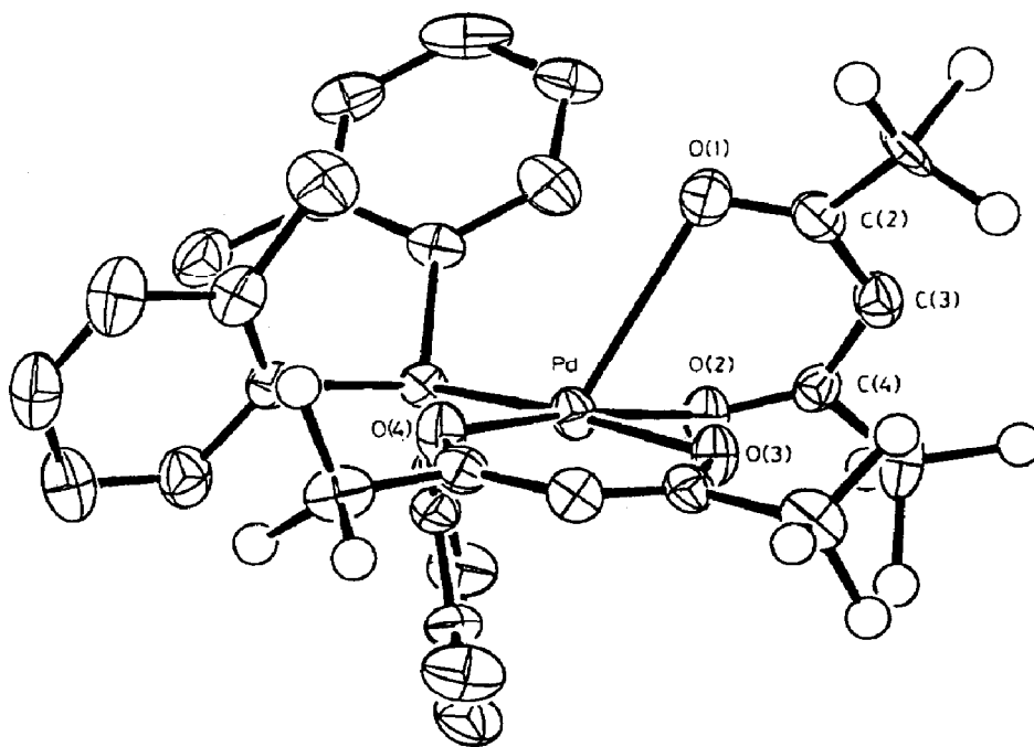
Fig. 7. The molecular structure of \text{Pd}(\text{hfac})_2\{\text{P}(\text{o-tolyl})_3\} [123]. \text{Pd}-\text{O}(1) = 2.797(6) Å, \text{Pd}-\text{O}(2) = 2.017(5) Å and \angle\text{O}(1)\text{PdO}(2) = 76.0(2)^\circ .
