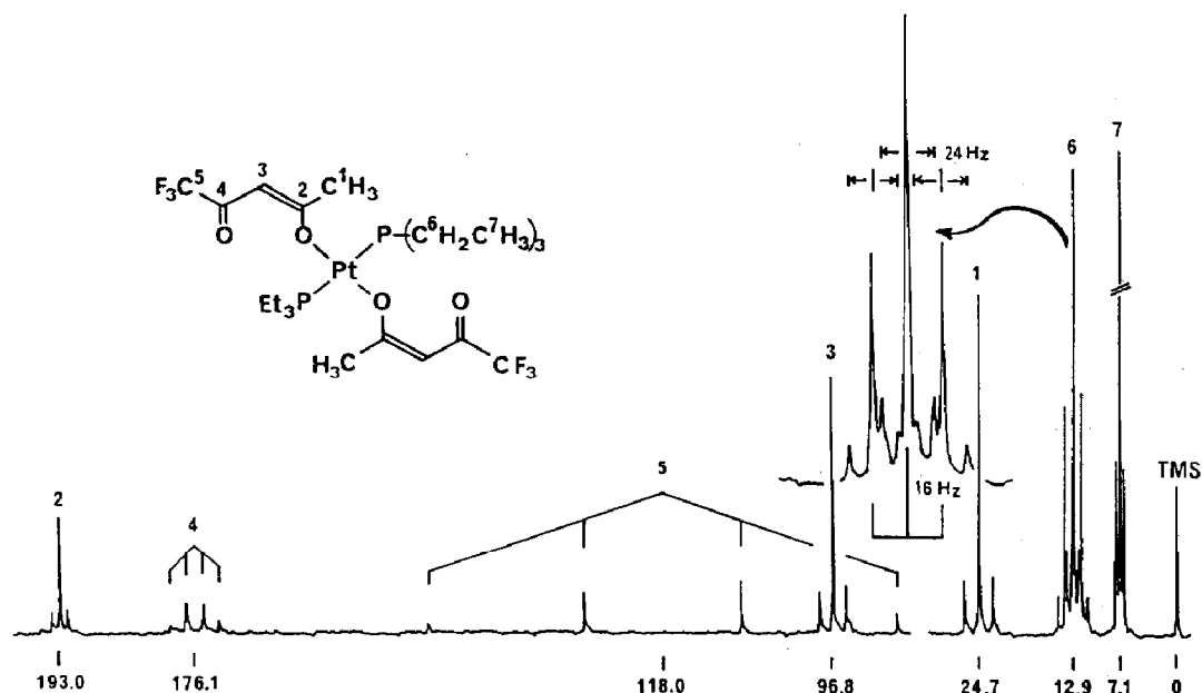
Fig. 5. ^{13}\text{C}\{^1\text{H}\} NMR spectrum at 15.04 MHz of \text{Pt}(\text{tfac-O})_2(\text{PEt}_3)_2 in \text{CDCl}_3 [95]. The J(\text{Pt-C}) values are 55, 28 and 55 Hz for \text{CH}_3 , CO and CH of tfac, and 24 and 15 Hz for \text{CH}_2 and \text{CH}_3 of \text{PEt}_3 , respectively. ^1J(\text{C-F}) = 292 Hz and ^2J(\text{C-F}) = 31 Hz.
