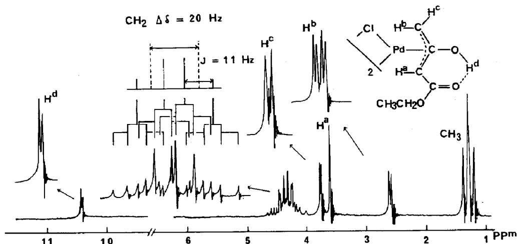
Fig. 8. ^1\text{H} NMR spectrum of [\text{PdCl}(\eta^3\text{-etag})]_2 in \text{CDCl}_3 [129]. J(\text{bc}) = 3.4 Hz, J(\text{bd}) = 1.2 Hz, and J(\text{CH}_3\text{-CH}_2) = 9.2 Hz.
