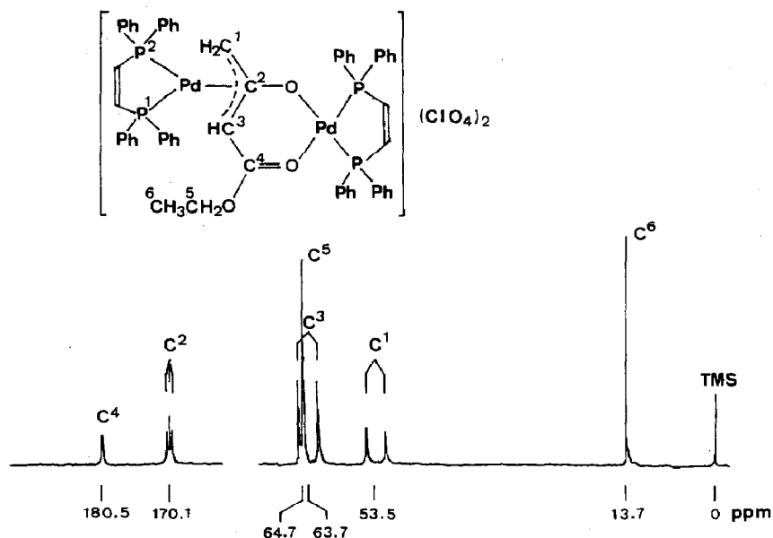
Fig. 12. ^{13}\text{C}\{^1\text{H}\} NMR signals at 15.04 MHz from the \text{etac}^{2-} ligand in [(\text{dpe})\text{Pd}(\eta^3\text{-etac}^{2-}\text{-O,O'})\text{Pd}(\text{dpe})](\text{ClO}_4)_2 in \text{acetone-}d_6 [141]. J(\text{P}^1\text{-C}^1) = 43 Hz, J(\text{P}^1\text{-C}^2) = J(\text{P}^2\text{-C}^2) = 6 Hz, and J(\text{P}^2\text{-C}^3) = 33 Hz.
