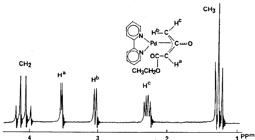
Fig. 10. ^1\text{H} NMR spectrum of \text{Pd}(\eta^3\text{-etac}^{2-})(\text{bpy}) in \text{CD}_2\text{Cl}_2 [129]. Signals from the bipyridine-ring protons are omitted. J(\text{bc}) = 4.4 Hz and J(\text{ac}) = 2.3 Hz.
